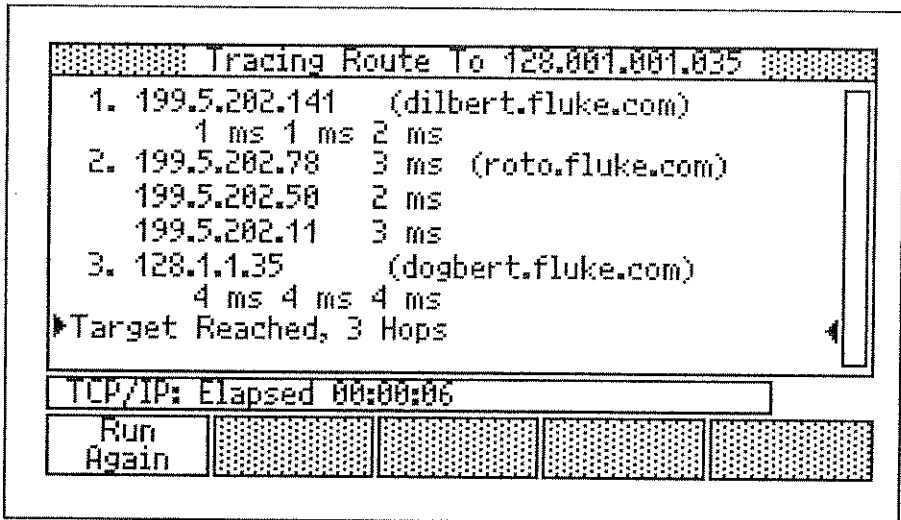
Figure 8-18. Different Routes Used
